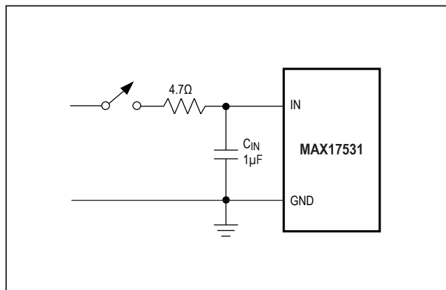
Figure 4. Transient Protection
