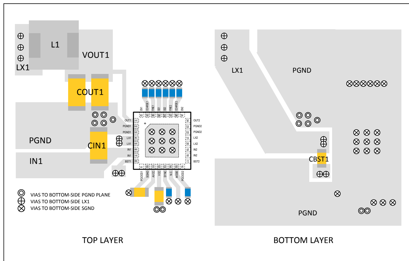
Figure 2. Recommended Layout
