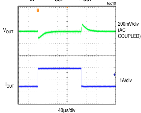
LOAD CURRENT TRANSIENT RESPONSE
