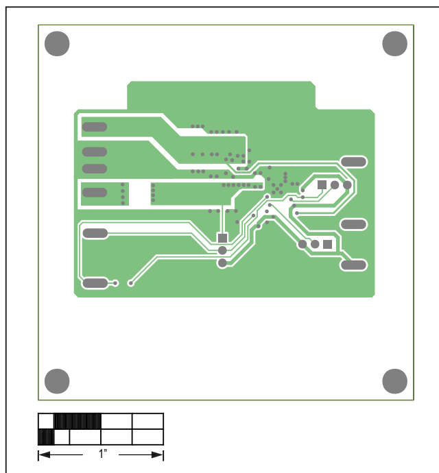
MAX17505EVKITBE# PCB Layout—Layer 3
