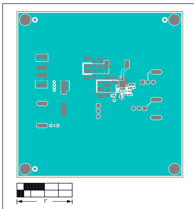
MAX17505EVKITBE# PCB Layout—Top Layer
