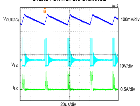
STEADY-STATE PERFORMANCE
