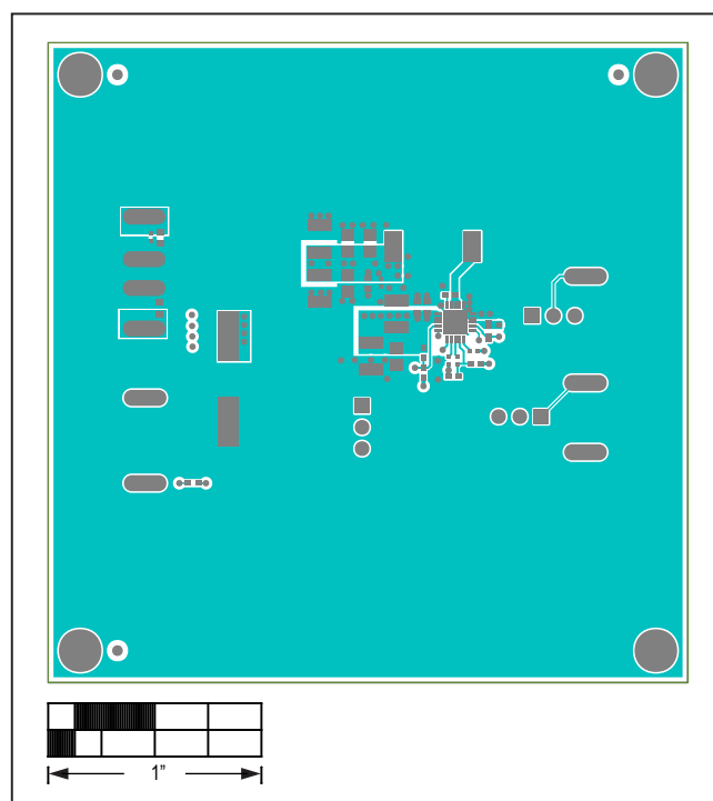
MAX17503EVKITBE# PCB Layout—Top Layer
