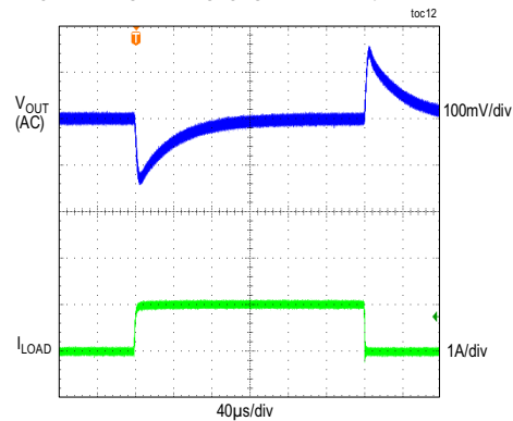
LOAD TRANSIENT RESPONSE BETWEEN 0A AND 1A
