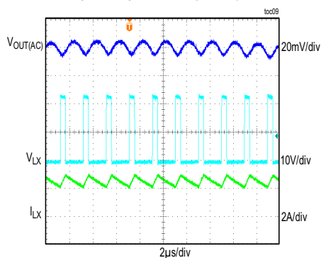
STEADY-STATE PERFORMANCE
