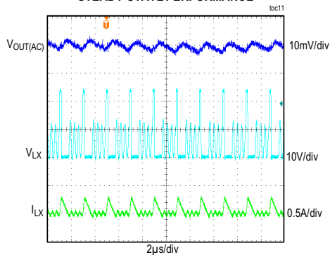
STEADY-STATE PERFORMANCE
