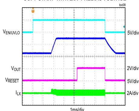
SOFT-START WITH 2.5V PREBIAS VOLTAGE
