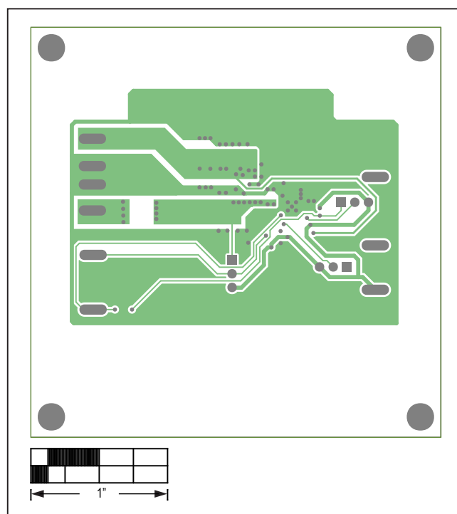
MAX17503EVKITBE# PCB Layout—Layer 3
