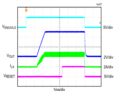
SOFT-START/SHUTDOWN THROUGH EN/UVLO
