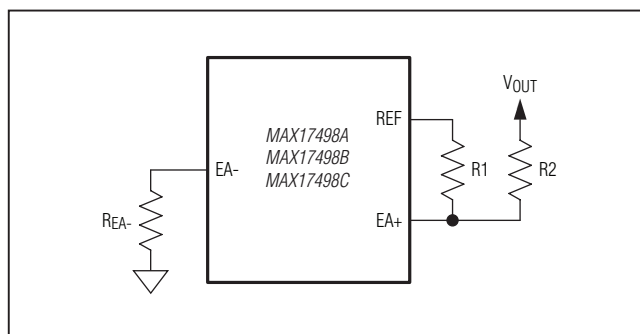
Figure 7. Programming the Negative Output Voltage
