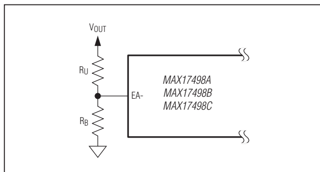
Figure 6. Programming the Positive Output Voltage
