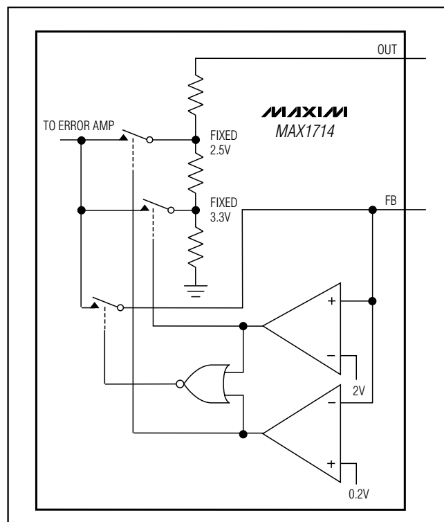
Figure 8. Feedback Mux
