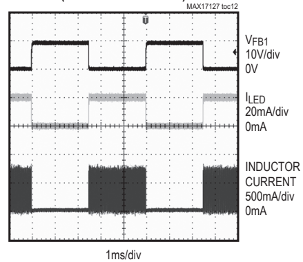
LED CURRENT WAVEFORMS (BRIGHTNESS = 50%)
