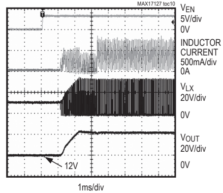
STARTUP WAVEFORMS (BRIGHTNESS = 100%)
