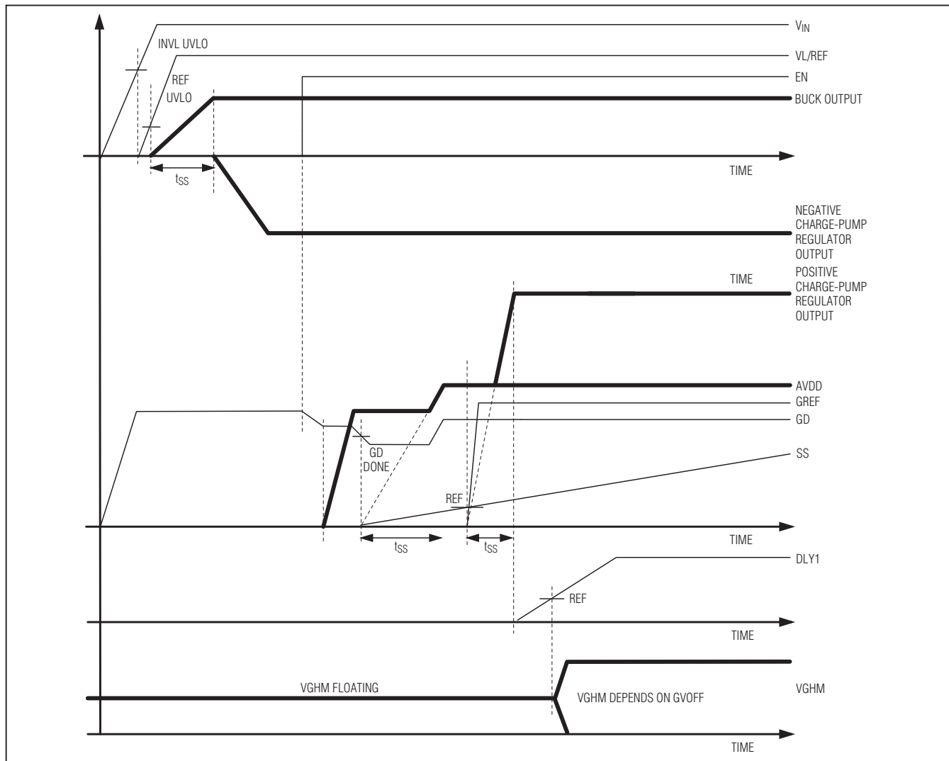
Figure 7. Power-Up Sequence
