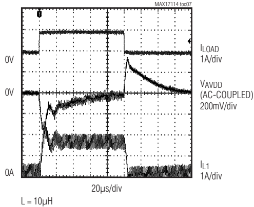
STEP-UP REGULATOR LOAD-TRANSIENT RESPONSE (0.1A TO 1.1mA)
