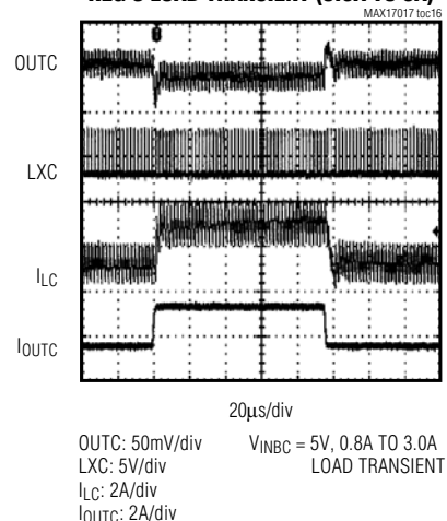
REG C LOAD TRANSIENT (0.8A TO 3A)
