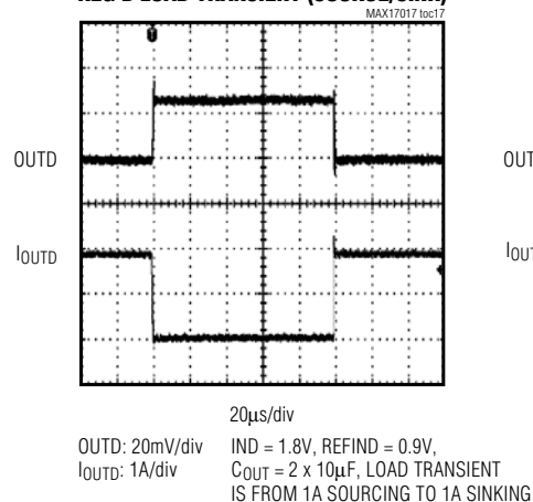
REG D LOAD TRANSIENT (SOURCE/SINK)
