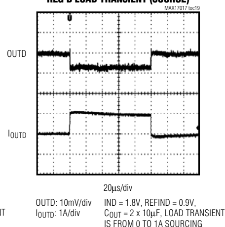
REG D LOAD TRANSIENT (SOURCE)
