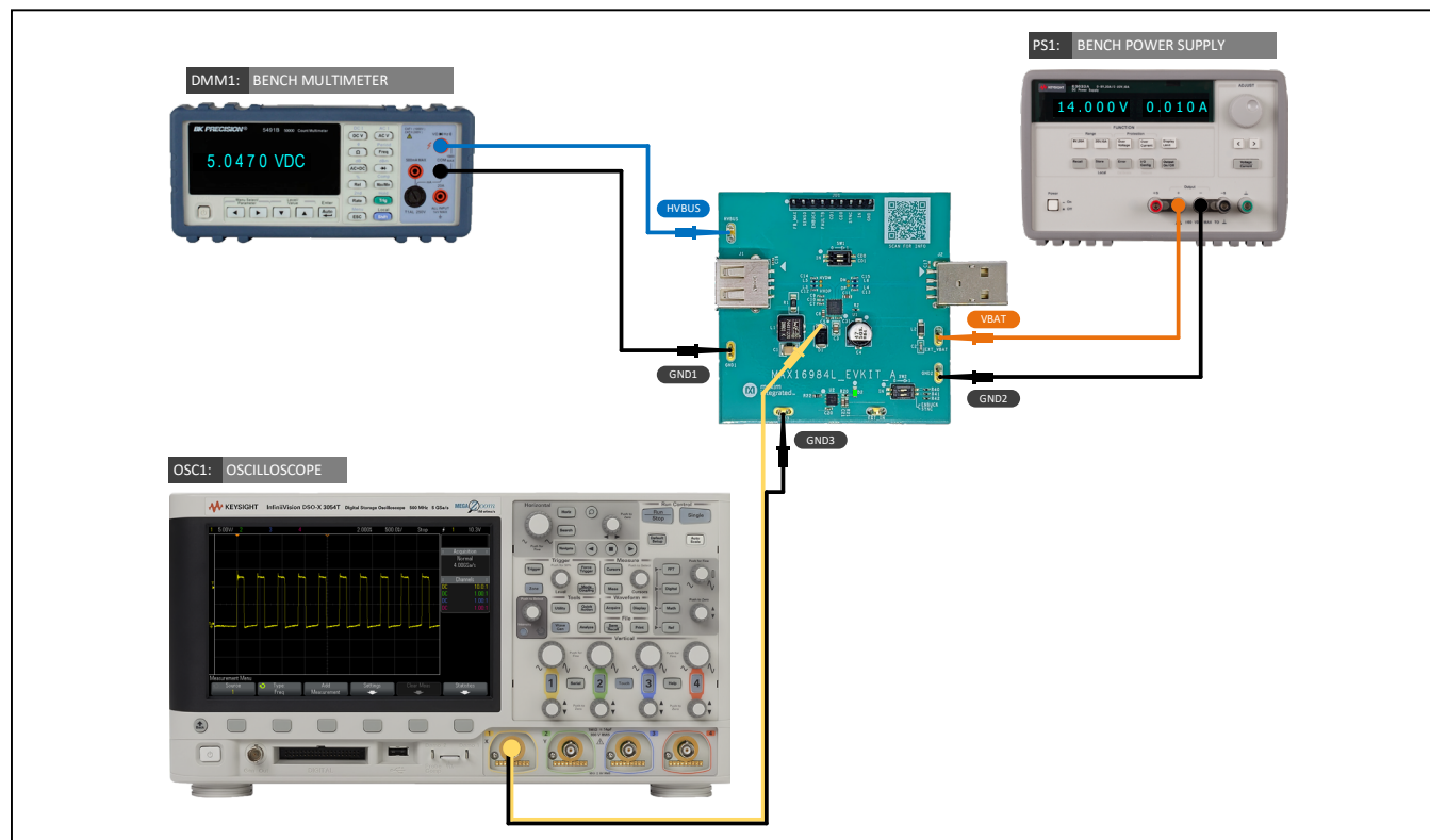
Figure 6. Test Setup for Buck FORCED PWM Mode
