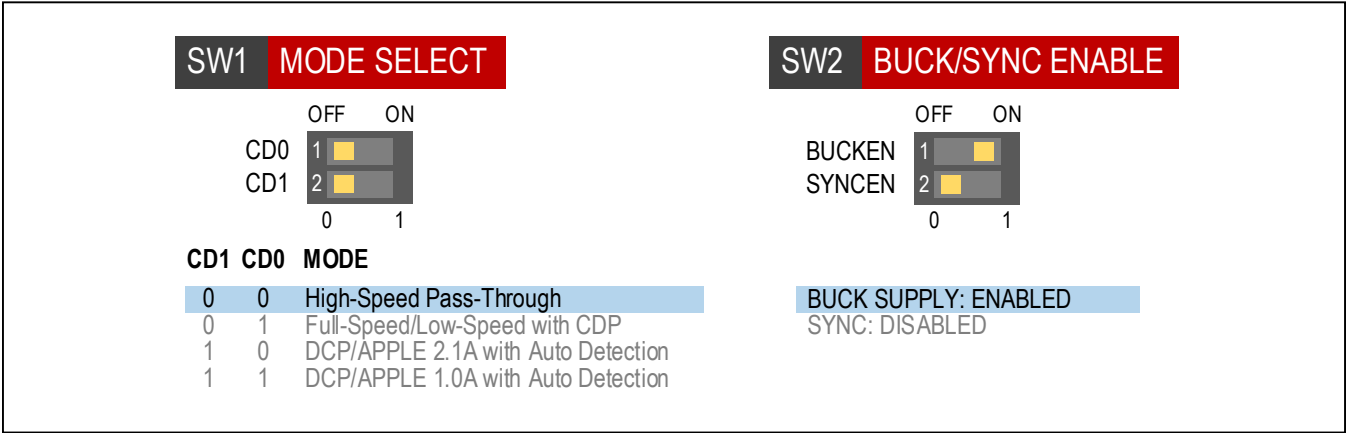
Figure 8. SW1 and SW2 Selections for SKIP Mode
