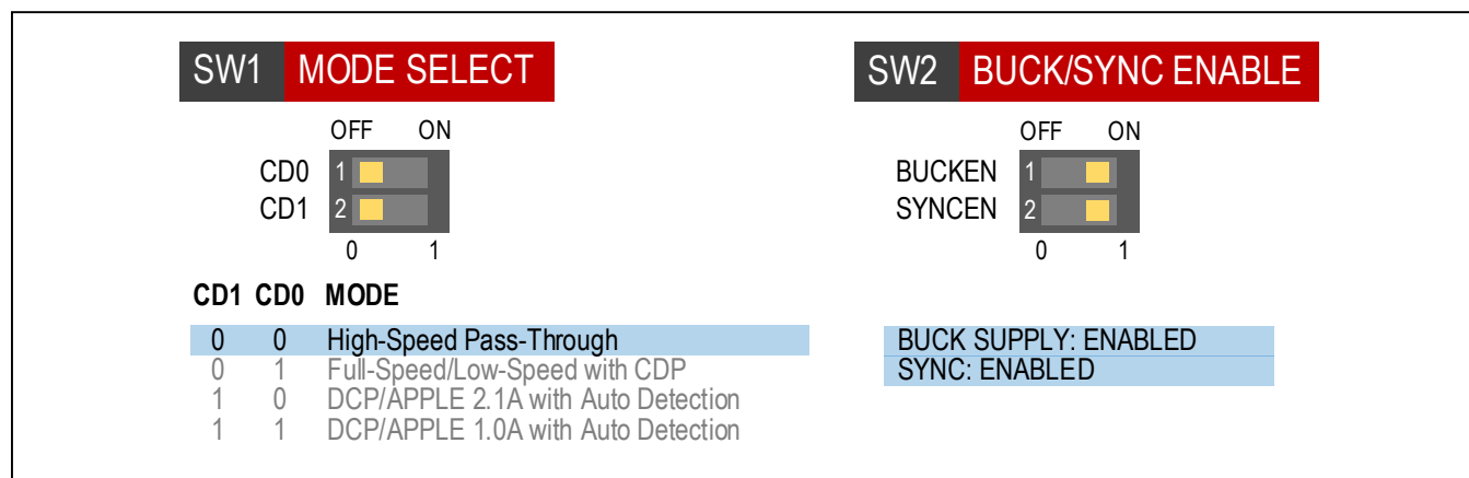
Figure 5. DIP Switch Selections for Buck Forced PWM Mode
