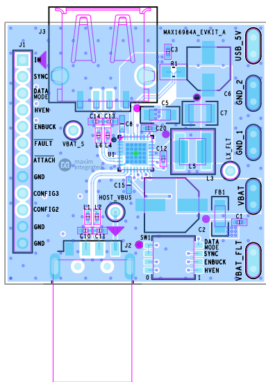
MAX16984A EV Kit PCB Layout—Top View
