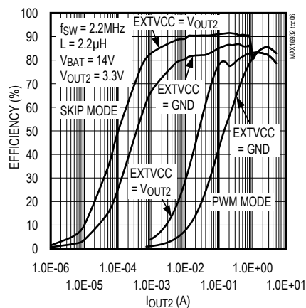
BUCK2 EFFICIENCY
