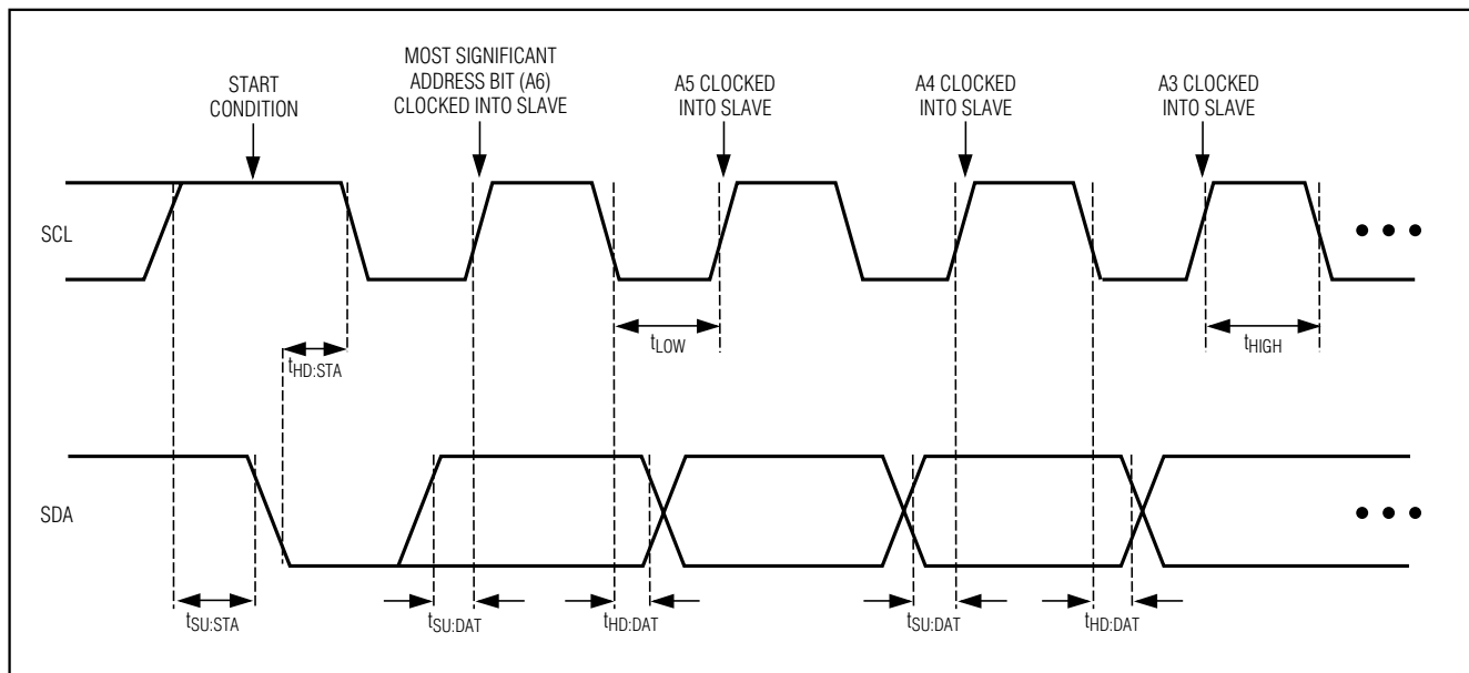
Figure 1. SMBus Serial-Interface Timing—Address
