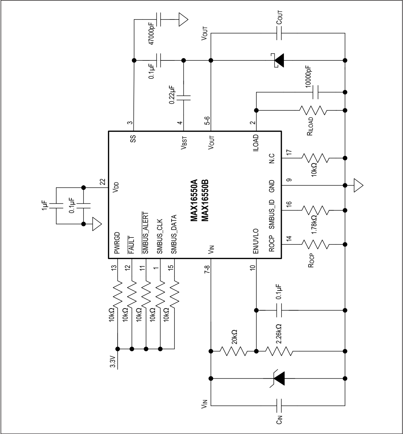
Figure 6. Reference Schematic
