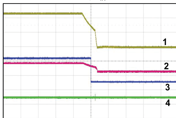
Shutdown Controlled by V_{IN} , 1Ω Resistive Load
