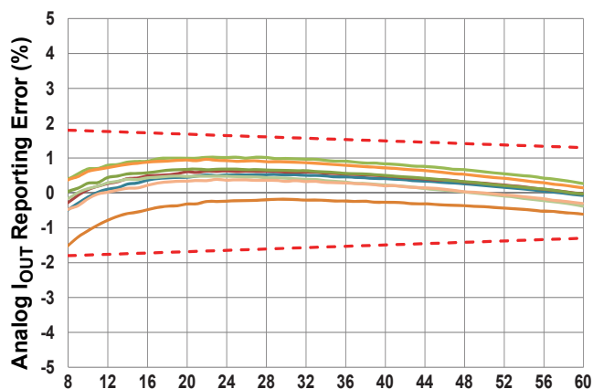
Analog I_{OUT} Reporting Accuracy
