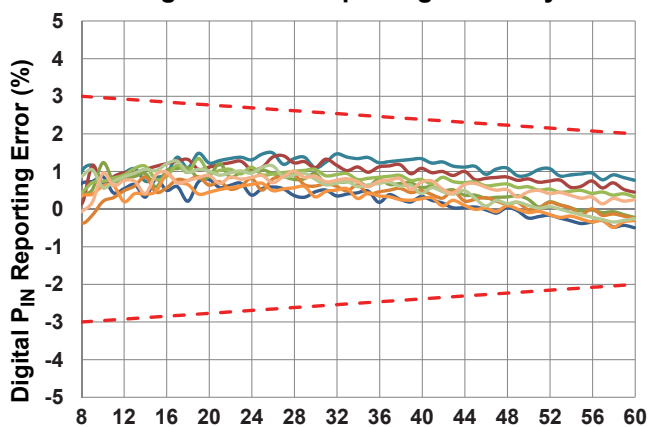
Digital Power Reporting Accuracy
