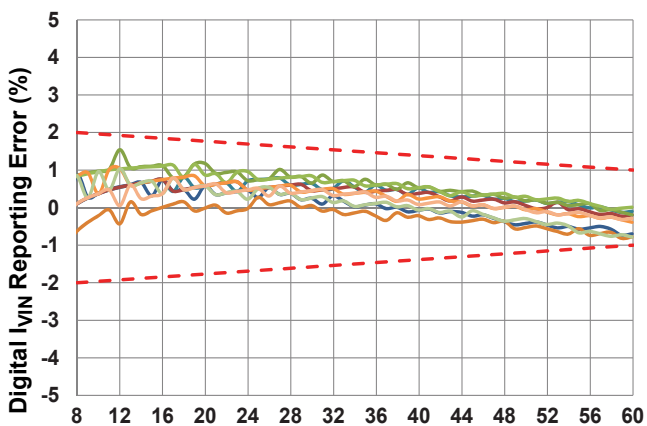
Digital I_{VIN} Reporting Accuracy
