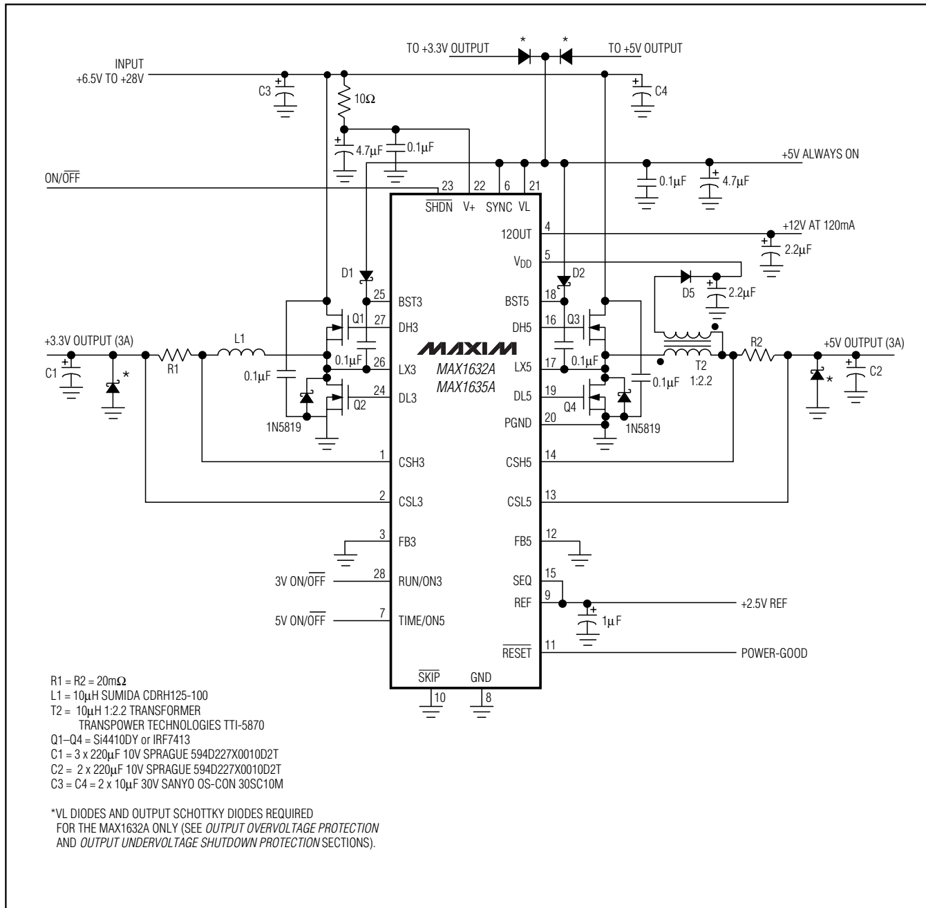
Figure 9. Triple-Output Application for High-Voltage Batteries (MAX1632A/MAX1635A)
