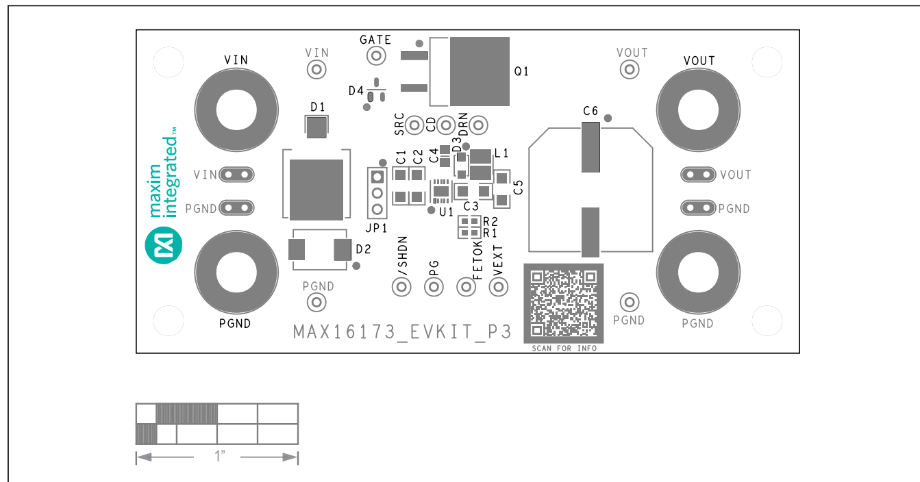
Figure 2. MAX16173 EV Kit Component Placement Guide—Component Side
