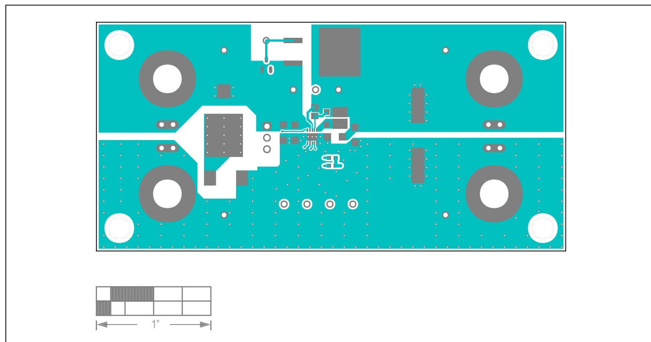
Figure 3. MAX16173 EV Kit PCB Layout—Component Side
