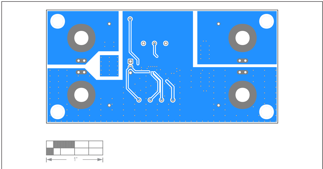
Figure 4. MAX16173 EV Kit PCB Layout—Bottom Side
