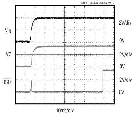
V7 AND R S0 STARTUP WAVEFORMS
