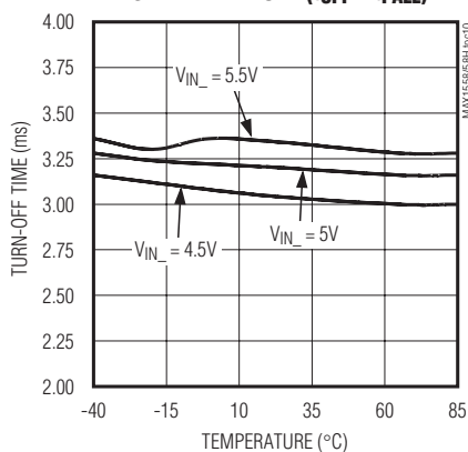
TURN-OFF TIME vs. TEMPERATURE ( t_{OFF} + t_{FALL} )
