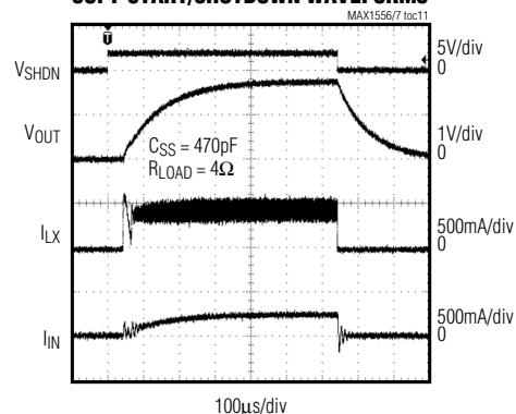
SOFT-START/SHUTDOWN WAVEFORMS
