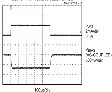
LOAD-TRANSIENT RESPONSE
