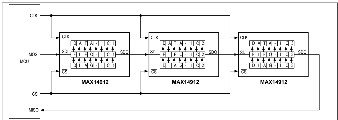
Figure 7. Daisy-Chain Connection
