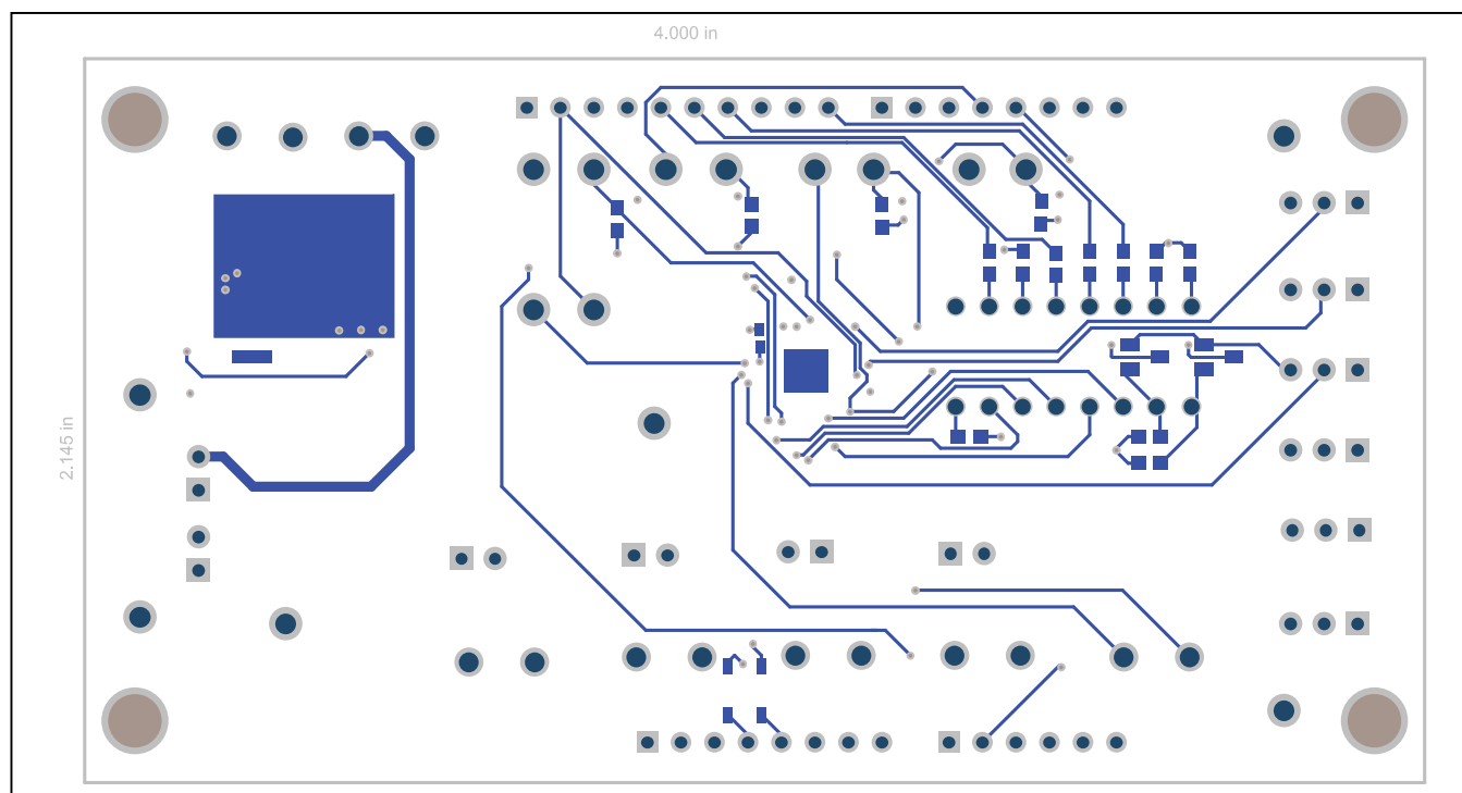
Figure 6. MAX14890E EV Kit PCB Layout—Bottom Layer
