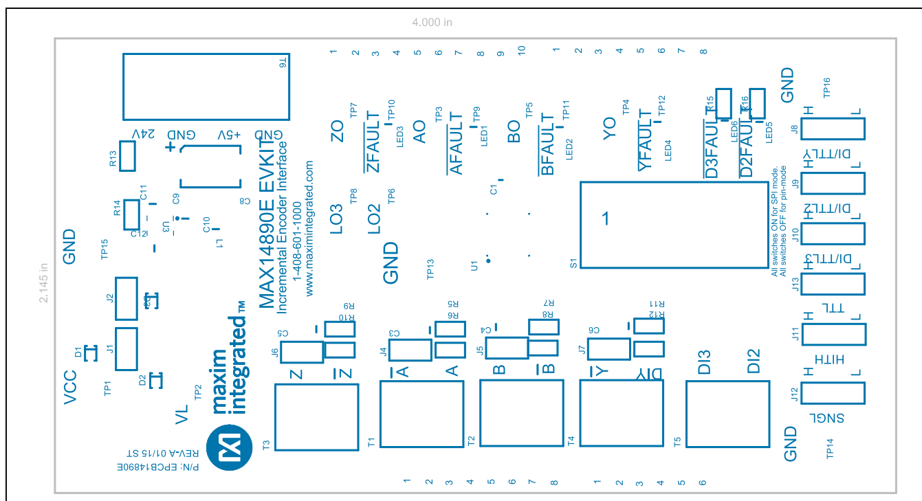
Figure 2. MAX14890E EV Kit Component Placement Guide—Top Silkscreen
