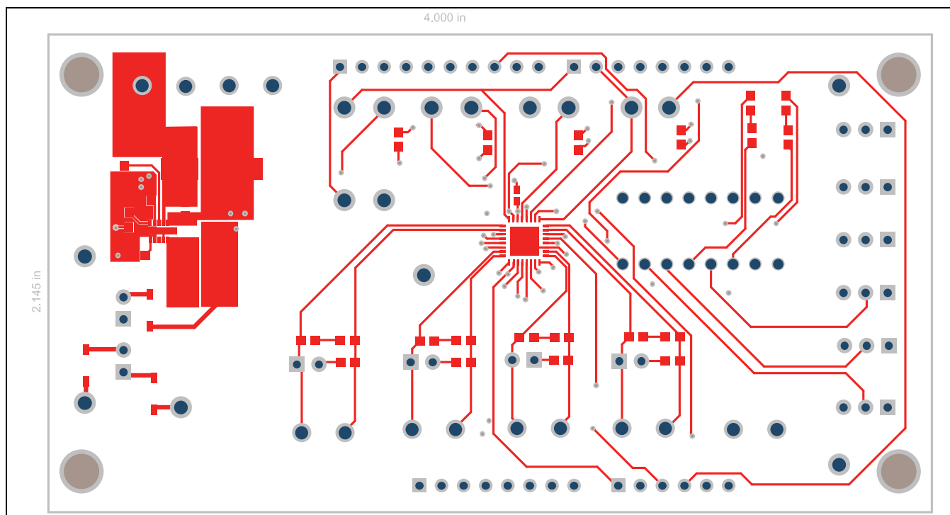
Figure 3. MAX14890E EV Kit PCB Layout—Top Layer
