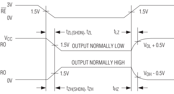
Figure 15. Receiver Enable and Disable Times (except MAX488E and MAX490E)
