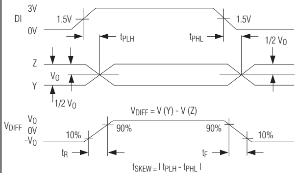
Figure 12. Driver Propagation Delays
