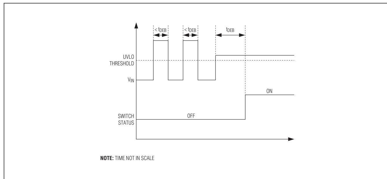
Figure 4. Debounce Timing
