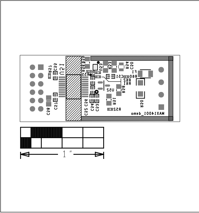
Figure 6. MAX14001PMB PCB Layout—Silkscreen Bottom
