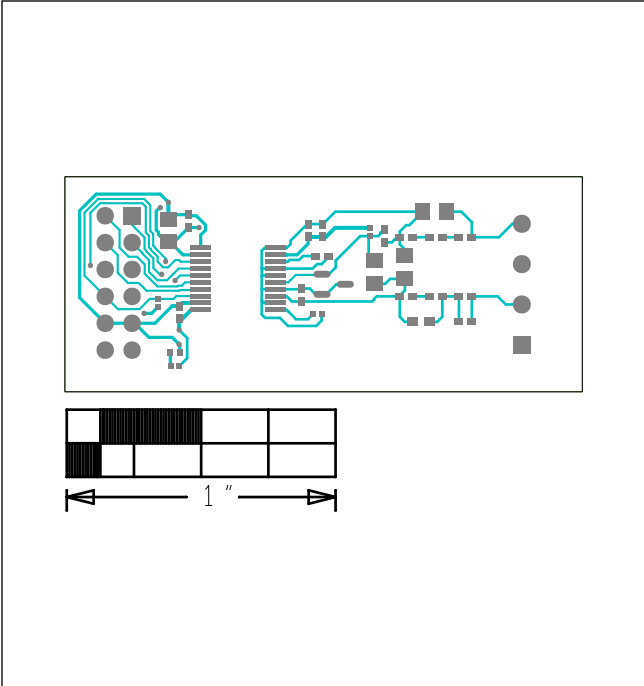
Figure 4. MAX14001PMB PCB Layout—Top
