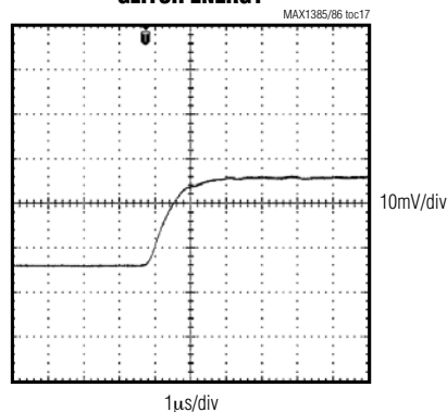
GLITCH ENERGY
