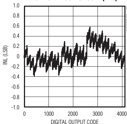
INTEGRAL NONLINEARITY vs. DIGITAL OUTPUT CODE (ADC)
