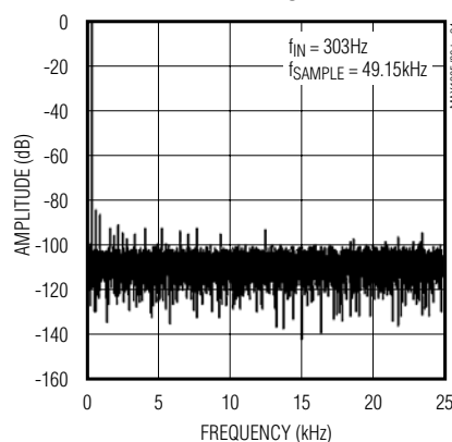
FFT PLOT
