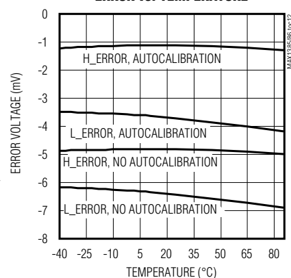
GATE_ OFFSET COMPENSATED ERROR vs. TEMPERATURE
