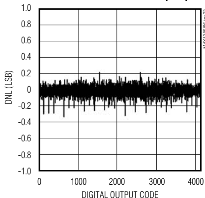
DIFFERENTIAL NONLINEARITY vs. DIGITAL OUTPUT CODE (ADC)
