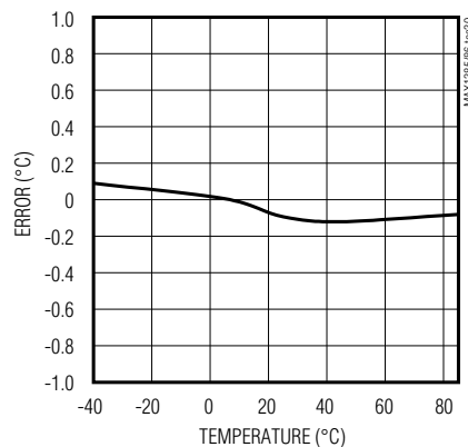
EXTERNAL TEMPERATURE SENSOR ERROR vs. TEMPERATURE
