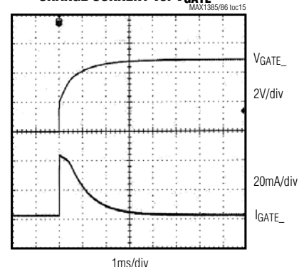
CHARGE CURRENT vs. V GATE
