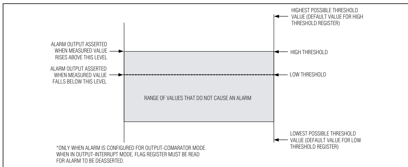
Figure 9. Hysteresis-Threshold-Mode Diagram
