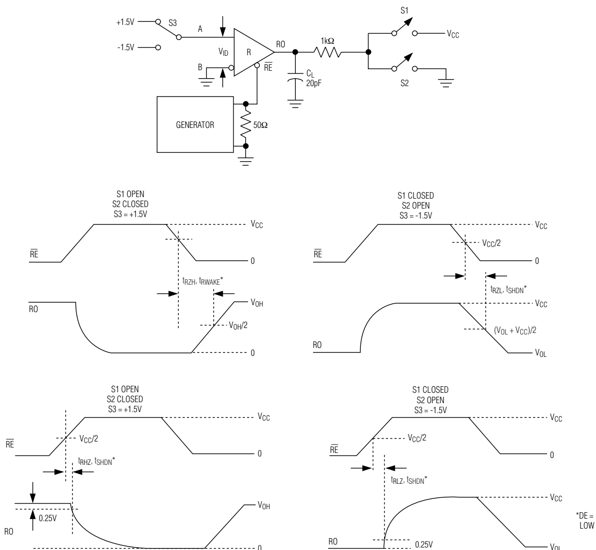
Figure 7. Receiver Enable and Disable Times
