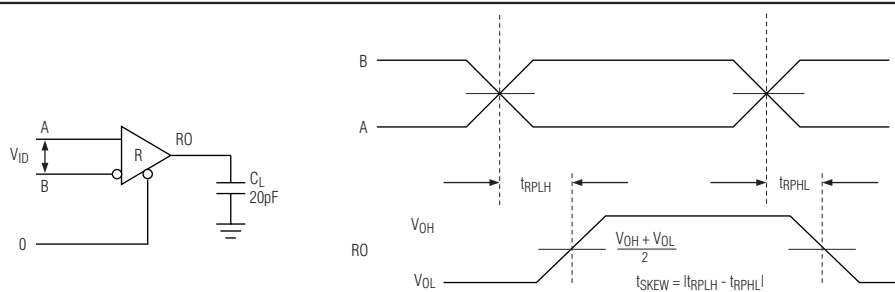
Figure 6. Receiver Propagation Delays
