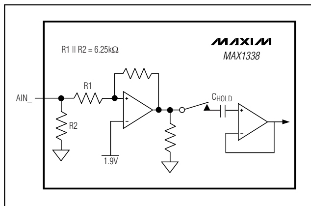
Figure 3. Simplified Typical Input Circuit
