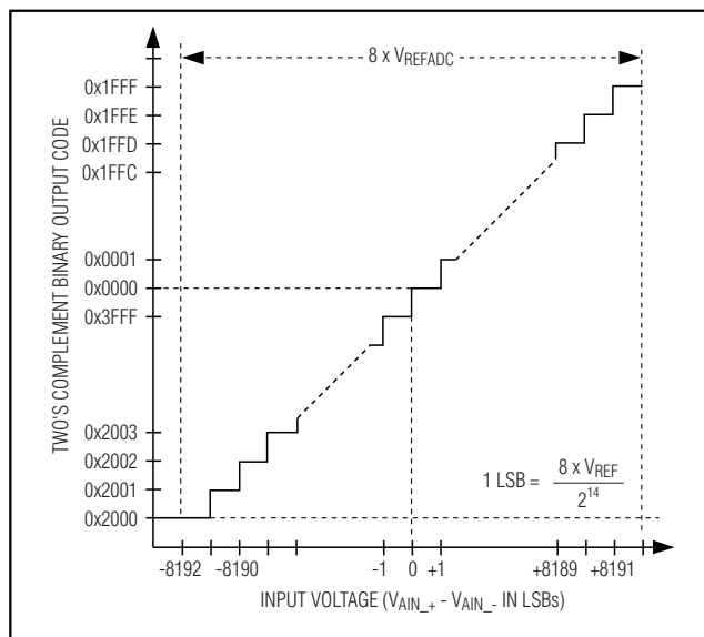
Figure 8. ±10V Transfer Function
