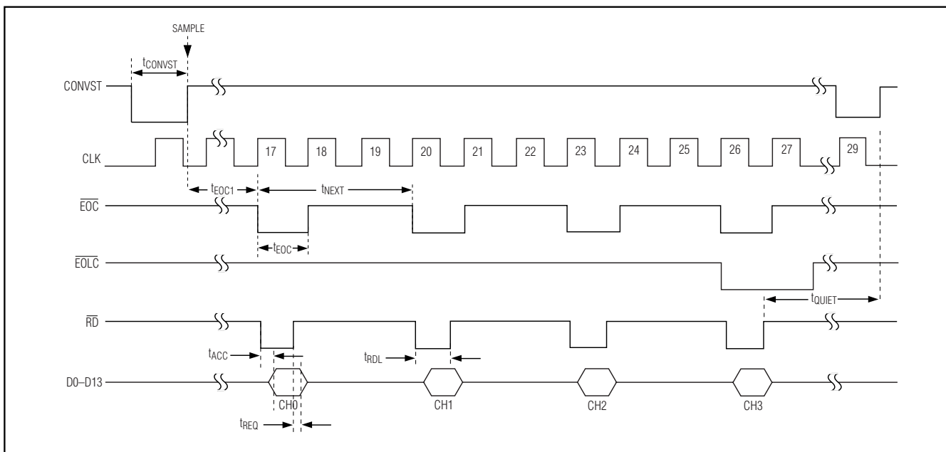
Figure 5. Reading During a Conversion—Internal or External Clock
