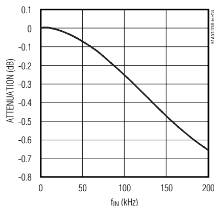
ANALOG INPUT BANDWIDTH
