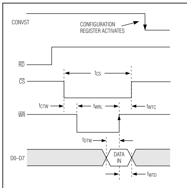
Figure 4. Write Timing
