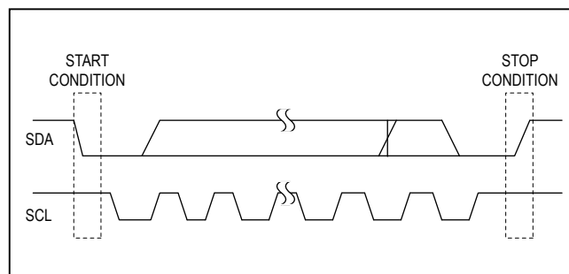
Figure 4. START/STOP Conditions
