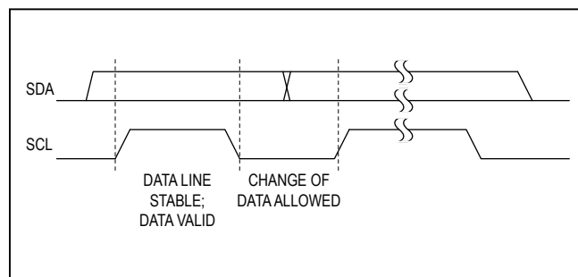
Figure 3. Bit Transfer
