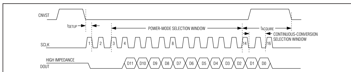
Figure 5. Interface-Timing Sequence
