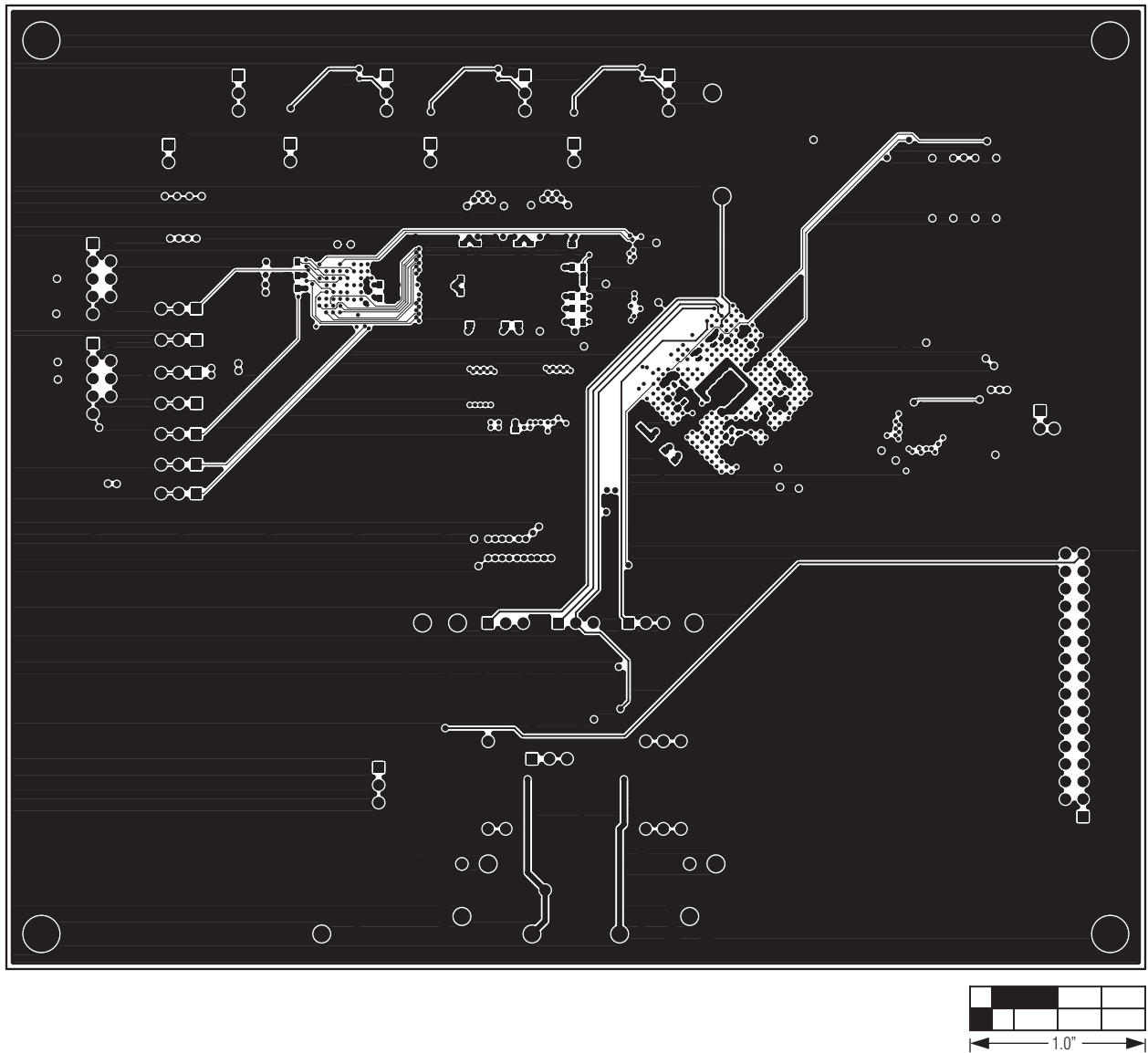
Figure 19. MAX11665 EV Kit PCB Layout—Bottom Side
