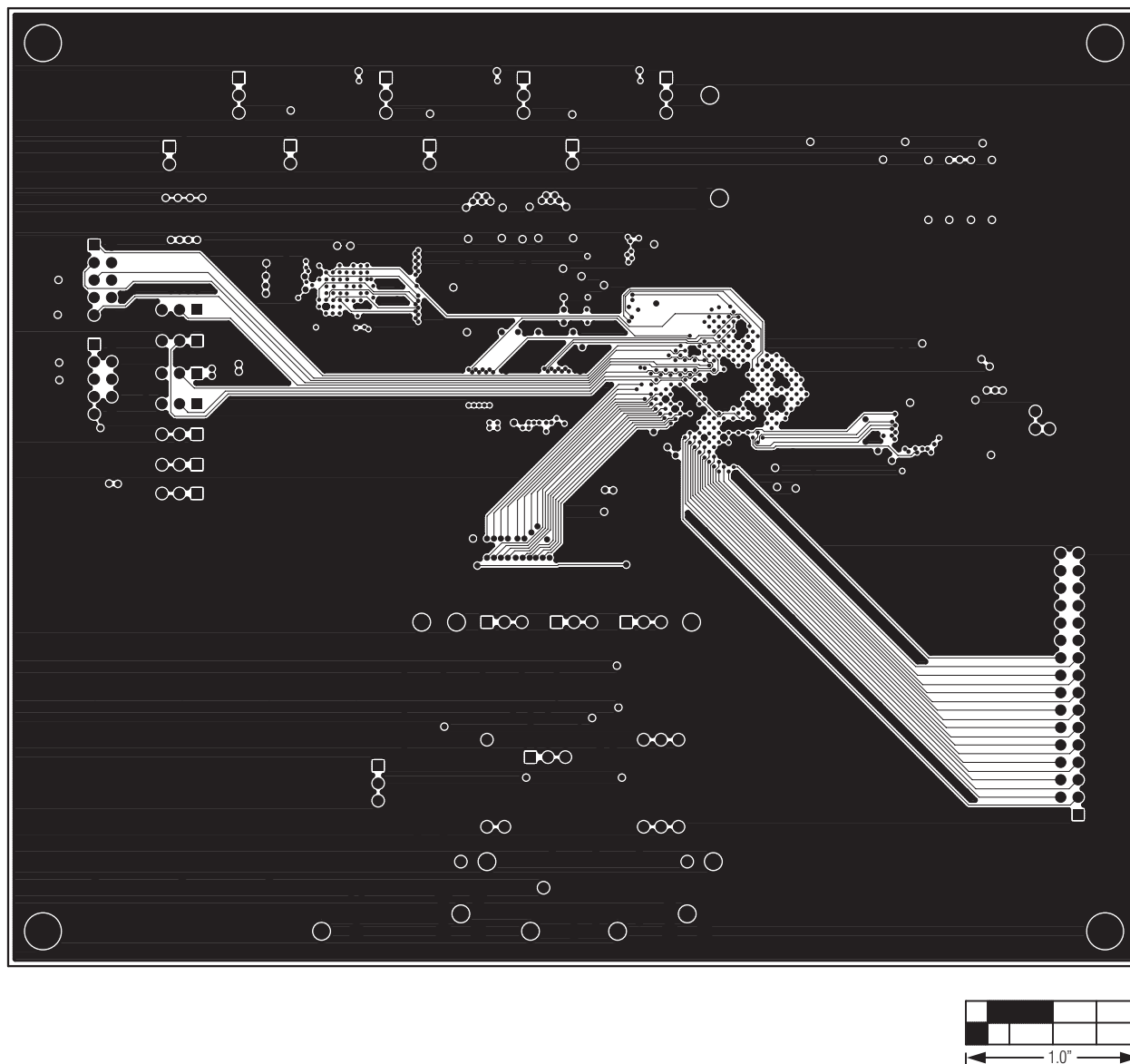
Figure 10. MAX11665 EV Kit PCB Layout—Layer 3
