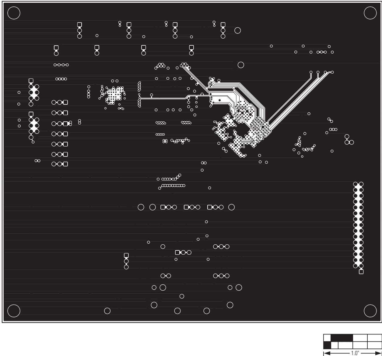
Figure 11. MAX11665 EV Kit PCB Layout—Layer 4
