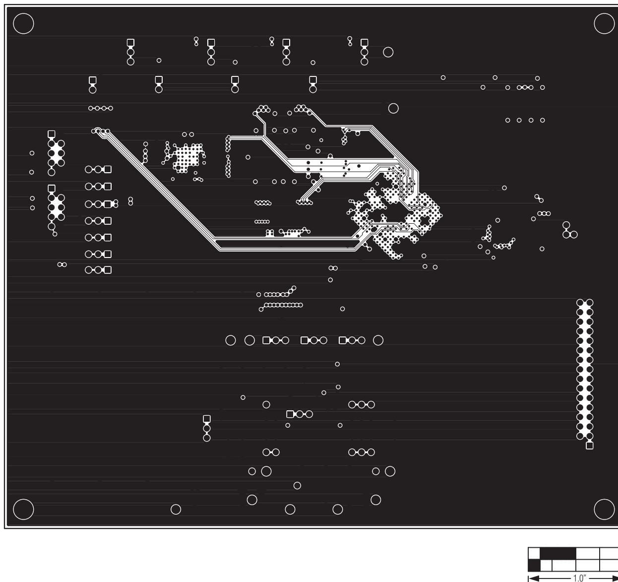
Figure 16. MAX11665 EV Kit PCB Layout—Layer 9
