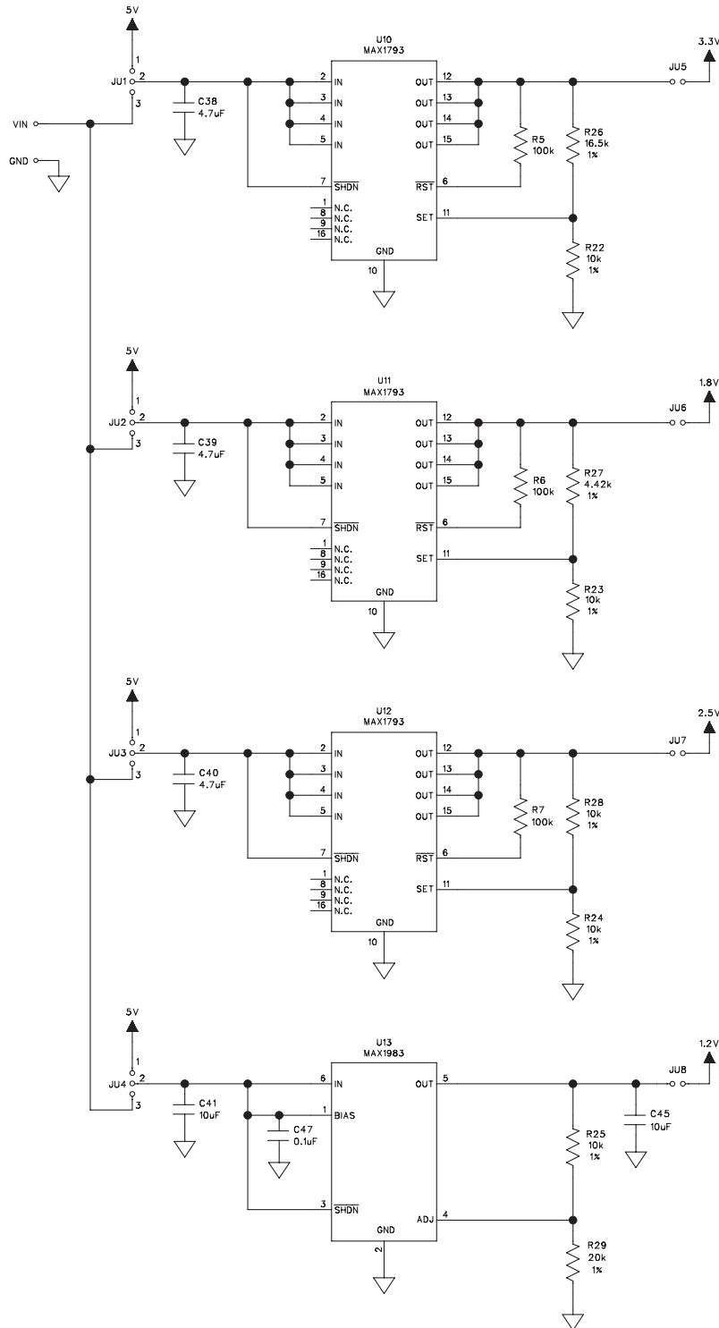
Figure 6k. MAX11665 EV Kit Schematic (Sheet 11 of 12)
