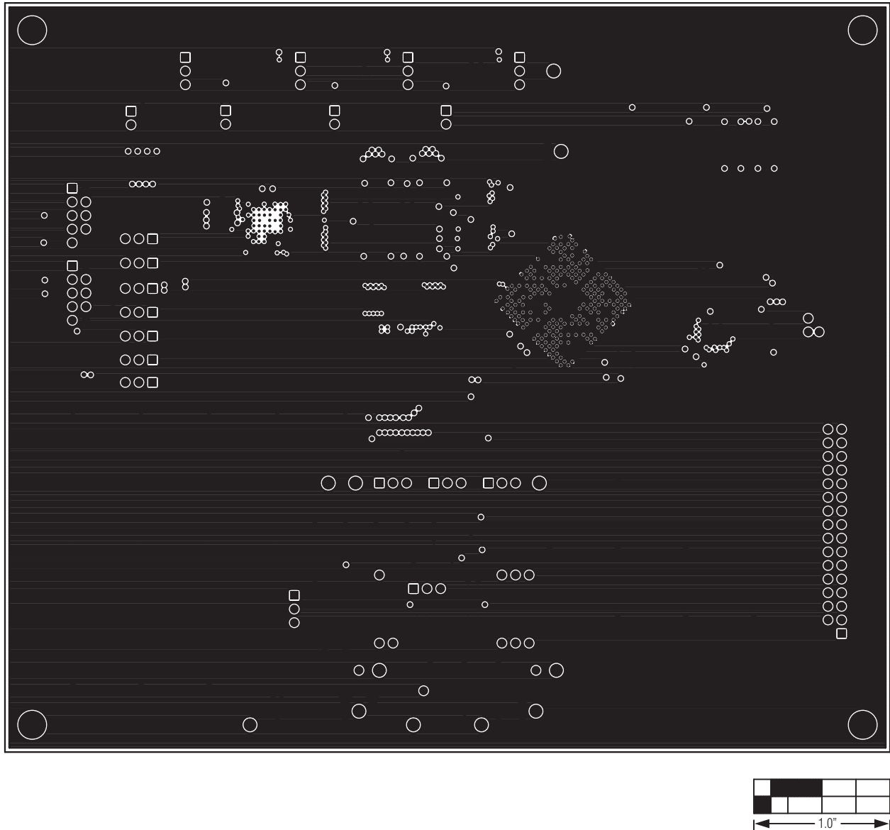
Figure 9. MAX11665 EV Kit PCB Layout—Layer 2
