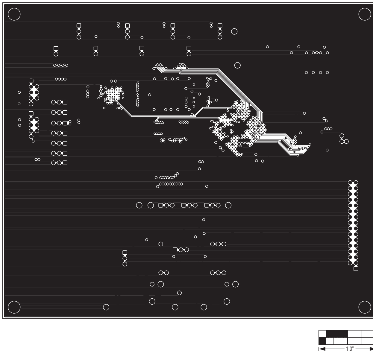
Figure 14. MAX11665 EV Kit PCB Layout—Layer 7
