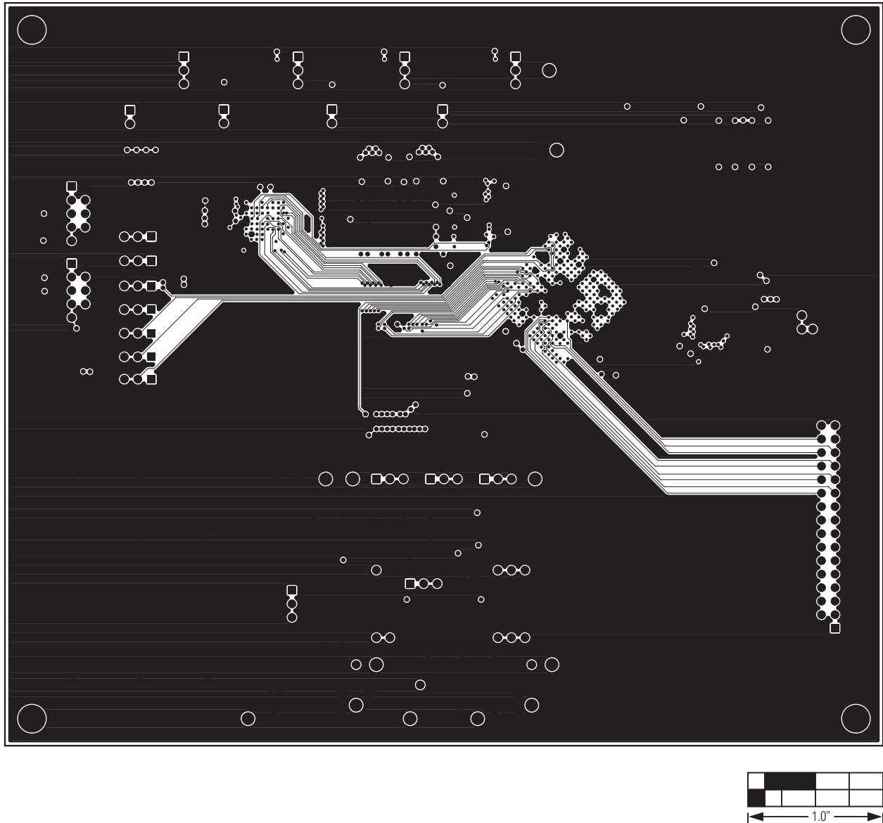
Figure 17. MAX11665 EV Kit PCB Layout—Layer 10
