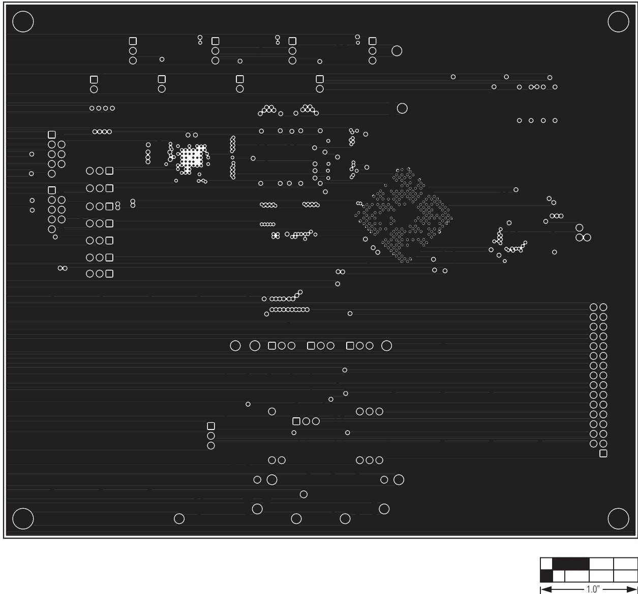
Figure 15. MAX11665 EV Kit PCB Layout—Layer 8
