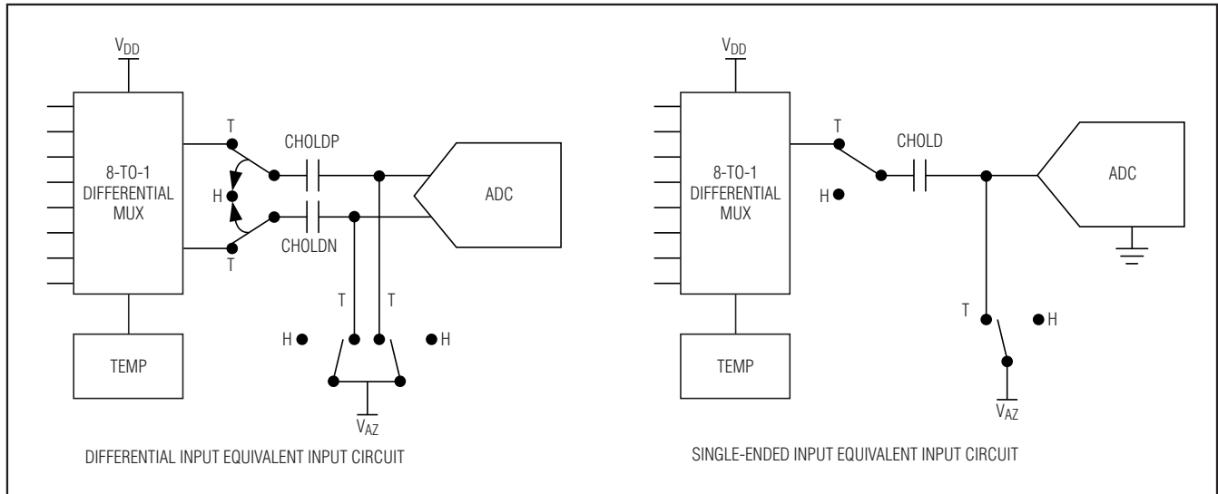
Figure 5. Single-Ended/Differential Input Equivalent Input Circuit
