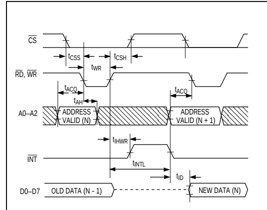
Figure 6. Pipelined Mode Timing ( \overline{WR} = \overline{RD} ) (MODE = 1)
