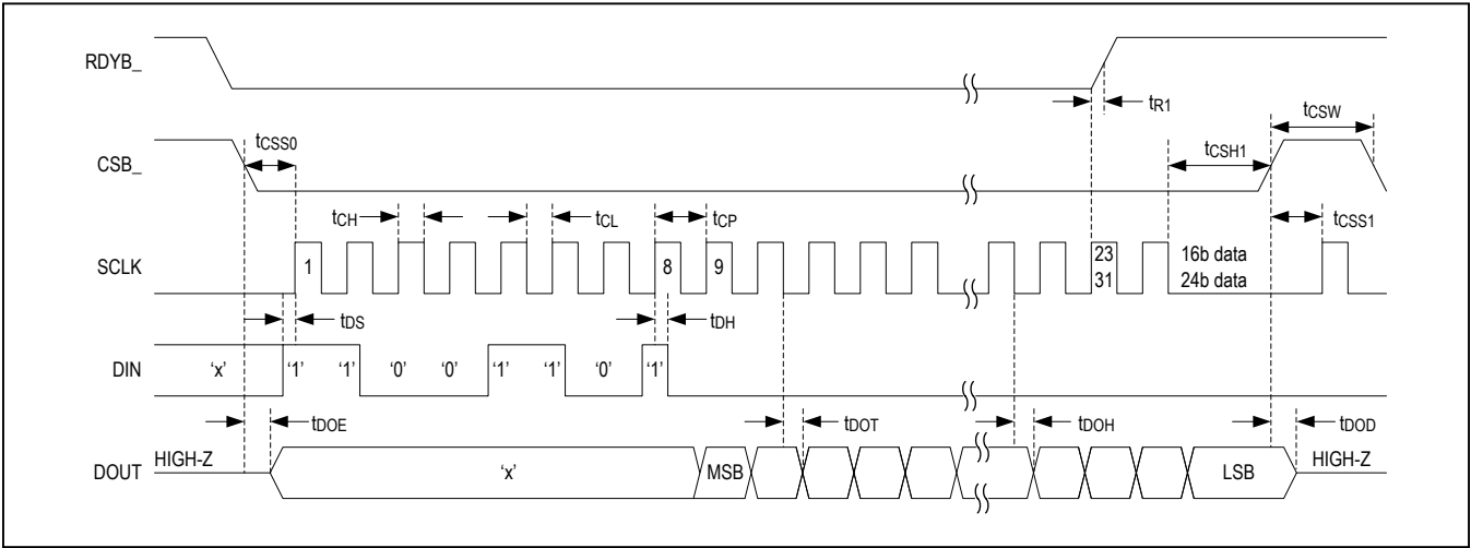
Figure 16. SPI Data Readout Timing Diagram
