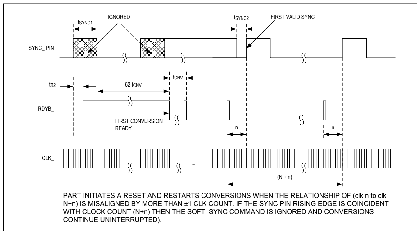
Figure 19. Synchronization Using Continuous Sync Mode Showing Relationship Between SYNC Pin and CLK Pin
