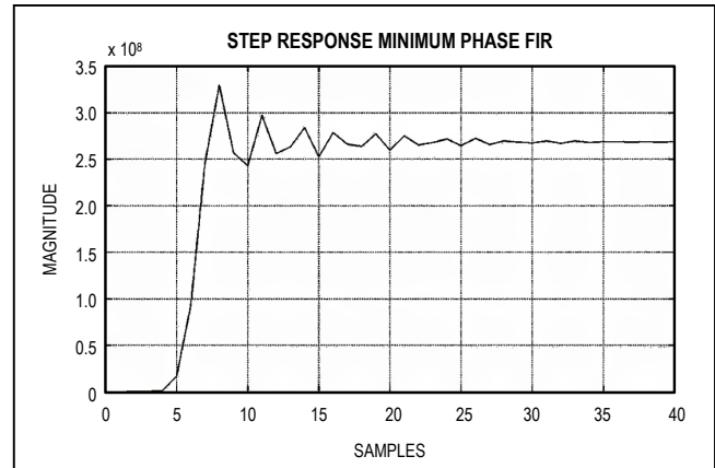
Figure 12. Step Response, Minimum Phase FIR
