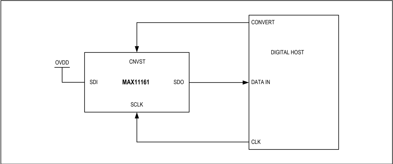
Figure 5. \overline{\text{CS}} Mode 3-Wire, No-Busy Indicator Connection Diagram (SDI High)
