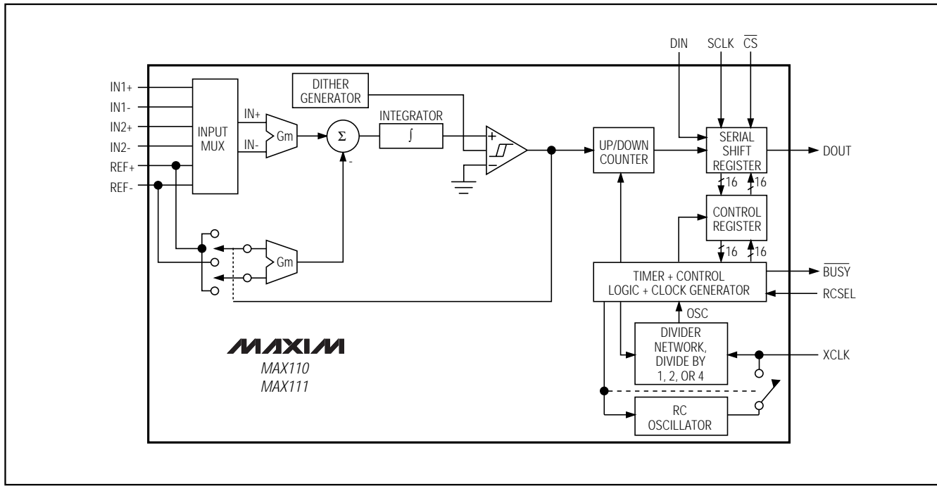
Figure 1. Functional Diagram
