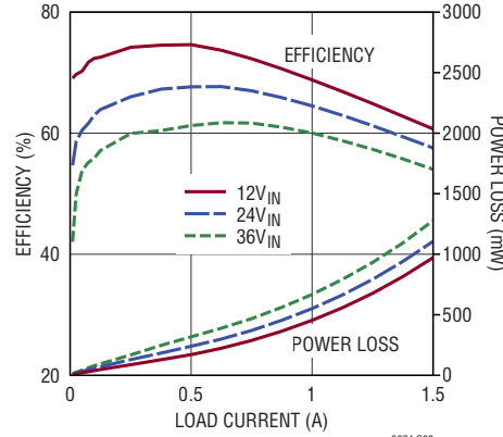
Efficiency and Power Loss, V_{OUT} = 1\text{V} , f_{SW} = 850\text{kHz}
