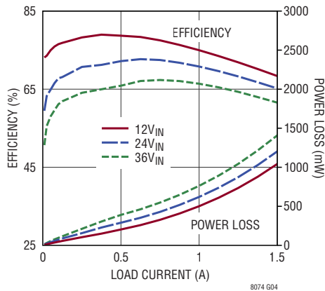
Efficiency and Power Loss, V_{OUT} = 1.5\text{V} , f_{SW} = 1\text{MHz}
