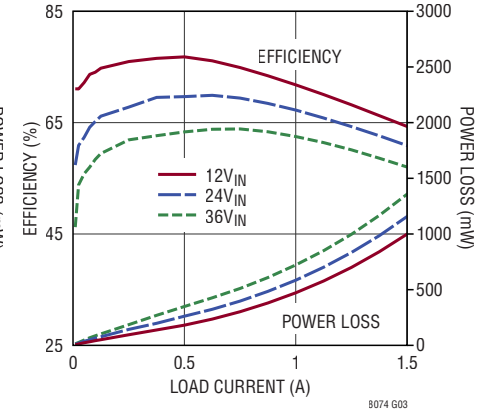
Efficiency and Power Loss, V_{OUT} = 1.2\text{V} , f_{SW} = 1\text{MHz}
