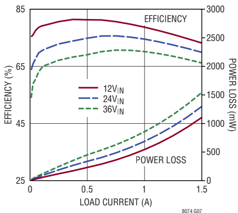
Efficiency and Power Loss, V_{OUT} = 2.5\text{V} , f_{SW} = 1.4\text{MHz}
