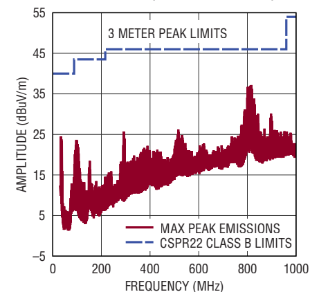
CISPR22 Class B Emissions DC2753A Demo Board V_{OUT} = 3.3\text{V} , 1.2A Load No EMI Filter (FB1, L1 Shorted)
