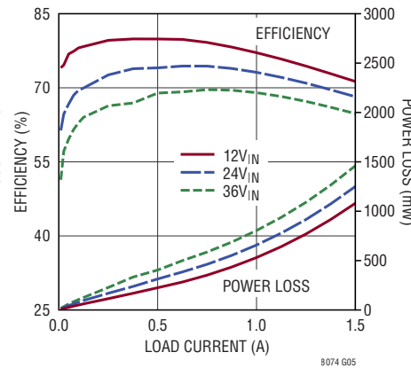
Efficiency and Power Loss, V_{OUT} = 1.8\text{V} , f_{SW} = 1\text{MHz}
