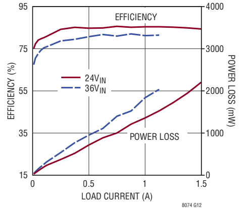
Efficiency and Power Loss, V_{OUT} = 8\text{V} , f_{SW} = 1.7\text{MHz}
