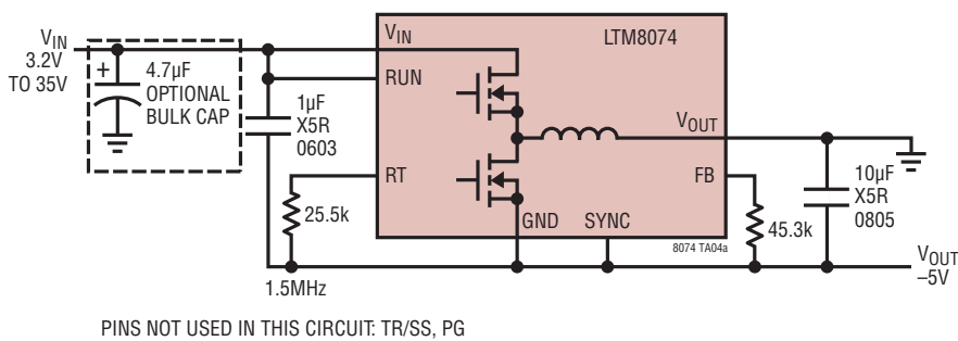
-5V OUT from 3.2V IN to 35V IN Positive to Negative Converter
