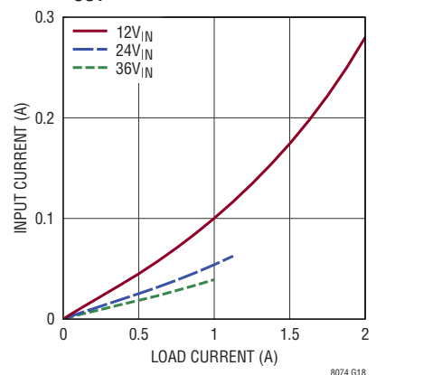
Input vs Load Current, V_{OUT} = 0.8\text{V}
