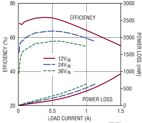
Efficiency and Power Loss, V_{OUT} = 0.8\text{V} , f_{SW} = 850\text{kHz}
