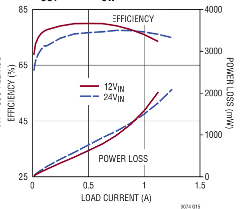
Efficiency and Power Loss, V_{OUT} = -5\text{V} , f_{SW} = 1.5\text{MHz}
