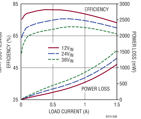
Efficiency and Power Loss, V_{OUT} = 2\text{V} , f_{SW} = 1.2\text{MHz}
