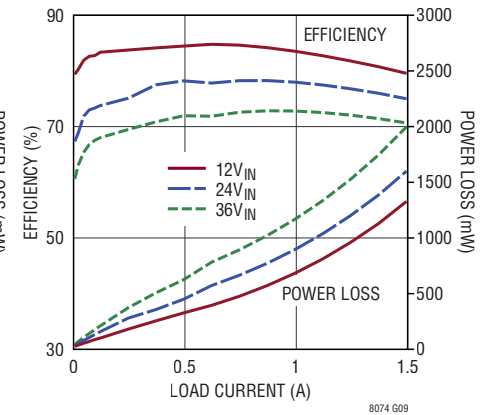
Efficiency and Power Loss, V_{OUT} = 3.3\text{V} , f_{SW} = 2\text{MHz}
