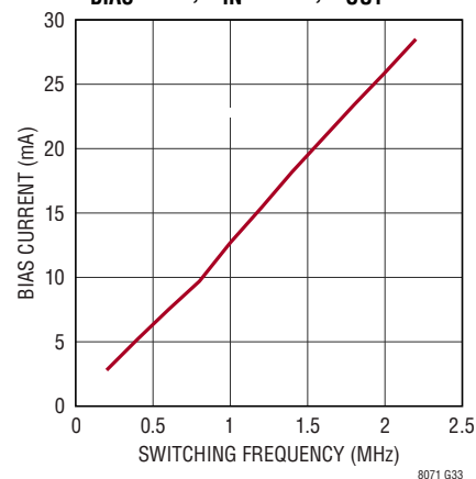
I_{BIAS} vs Switching Frequency V_{BIAS} = 5\text{V} , V_{IN} = 24\text{V} , V_{OUT} = 5\text{V}
