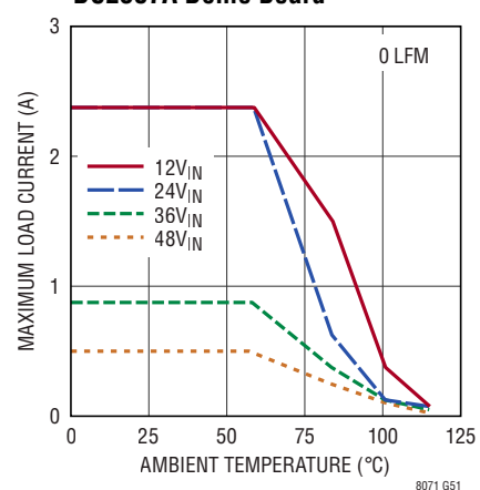
Derating, V_{OUT} = -12\text{V} , BIAS Tied to LTM8071 GND DC2387A Demo Board
