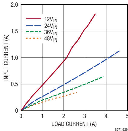
Input vs Load Current V_{OUT} = -15\text{V} BIAS Tied to LTM8071 GND
