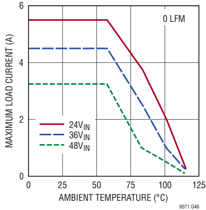
Derating, V_{OUT} = -3.3\text{V} , BIAS Tied to LTM8071 GND DC2387A Demo Board
