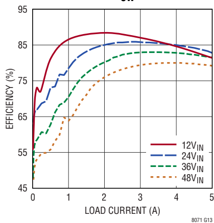
Efficiency vs Load Current V_{OUT} = -12\text{V} , BIAS Tied to LTM8071 GND, f_{SW} = 1.4\text{MHz}
