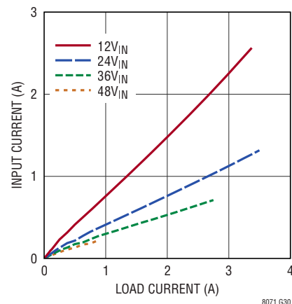
Input vs Load Current V_{OUT} = -8\text{V} BIAS Tied to LTM8071 GND
