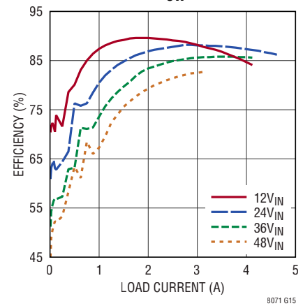
Efficiency vs Load Current V_{OUT} = -8\text{V} , BIAS Tied to LTM8071 GND, f_{SW} = 1.2\text{MHz}
