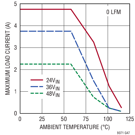
Derating, V_{OUT} = -5\text{V} , BIAS Tied to LTM8071 GND DC2387A Demo Board
