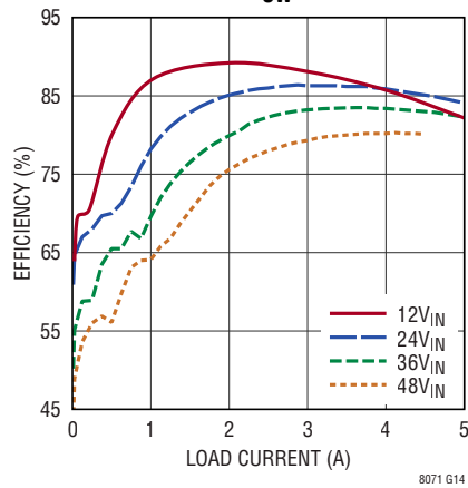
Efficiency vs Load Current V_{OUT} = -15\text{V} , BIAS Tied to LTM8071 GND, f_{SW} = 1.8\text{MHz}
