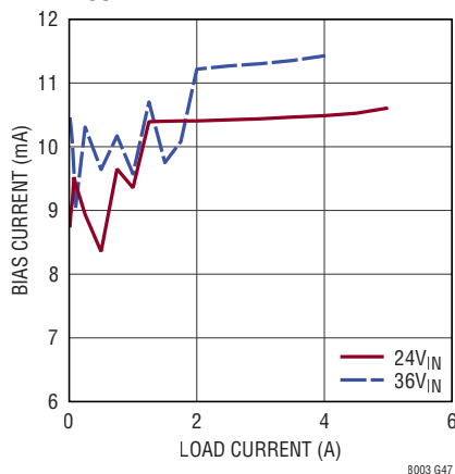
BIAS Current vs Load Current V_{OUT} = 15\text{V} , \text{BIAS} = 5\text{V}
