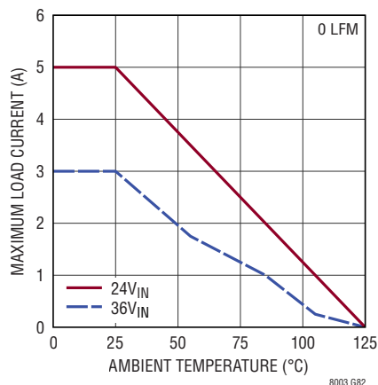
Derating, I-Grade, V_{OUT} = -8\text{V} , BIAS Tied to LTM8003 GND, DC2416A Demo Board
