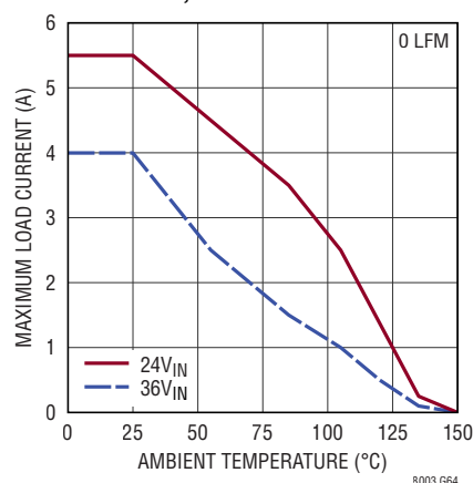
Derating, H-Grade, V_{OUT} = -8\text{V} , BIAS Tied to LTM8003 GND, DC2416A Demo Board
