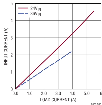
Input vs Load Current V_{OUT} = -8\text{V} , BIAS Tied to LTM8003 GND
