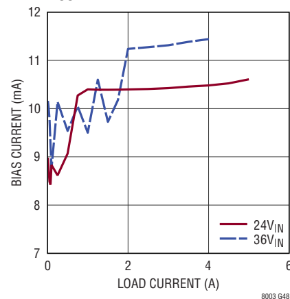
BIAS Current vs Load Current V_{OUT} = 18\text{V} , \text{BIAS} = 5\text{V}
