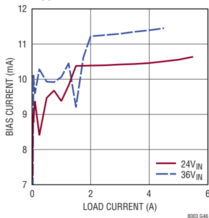
BIAS Current vs Load Current V_{OUT} = 12\text{V} , \text{BIAS} = 5\text{V}
