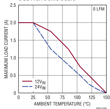
Derating, H-Grade, V_{OUT} = -15\text{V} , BIAS Tied to LTM8003 GND, DC2416A Demo Board
