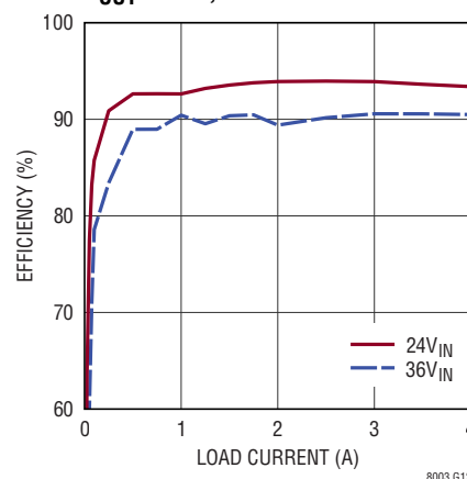
Efficiency vs Load Current, V_{OUT} = -8\text{V} , BIAS Tied to LTM8003 GND
