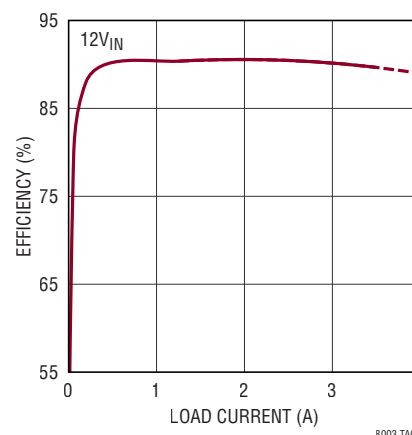
Efficiency, V OUT = 5V
