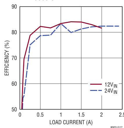
Efficiency vs Load Current, V_{OUT} = -15\text{V} , BIAS Tied to LTM8003 GND
