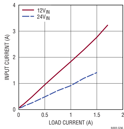
Input vs Load Current V_{OUT} = -18\text{V} , BIAS Tied to LTM8003 GND
