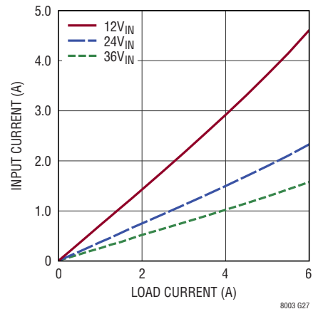
Input vs Load Current V_{OUT} = 8\text{V} , BIAS = 5V
