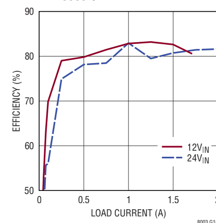
Efficiency vs Load Current, V_{OUT} = -18\text{V} , BIAS Tied to LTM8003 GND
