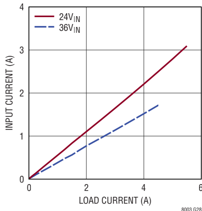
Input vs Load Current V_{OUT} = -3.3\text{V} , BIAS Tied to LTM8003 GND
