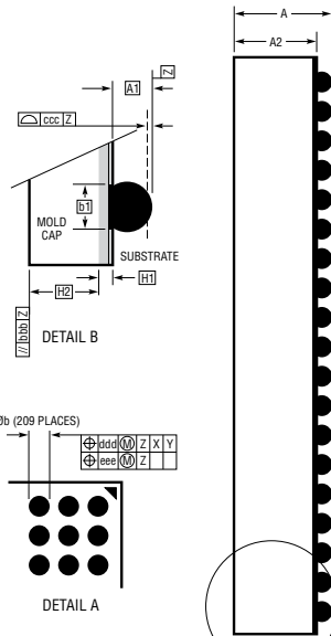
DETAIL B PACKAGE SIDE VIEW
