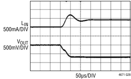
Short-Circuit Waveform with No Load Current Exist
