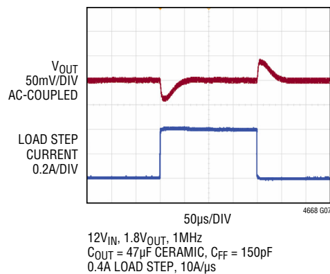
1.8V Output Transient Response
