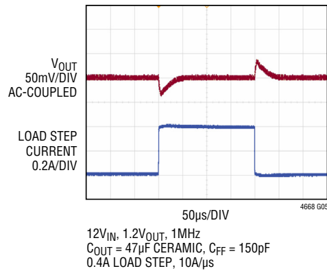
1.2V Output Transient Response
