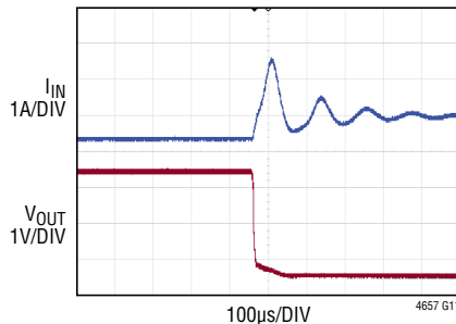
Short-Circuit with No Load Applied
