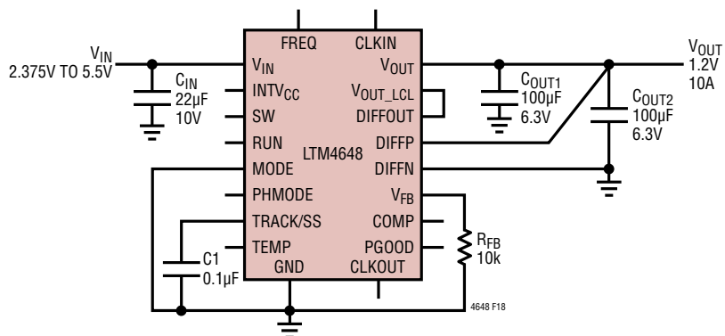
Figure 18. 2.375V to 5.5V IN , 1.2V at 10A Design
