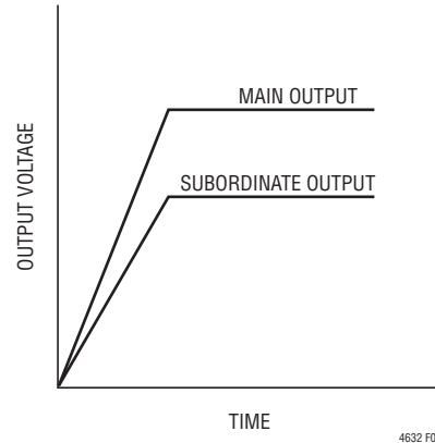
Figure 5. Output Ratiometric Tracking Waveform
