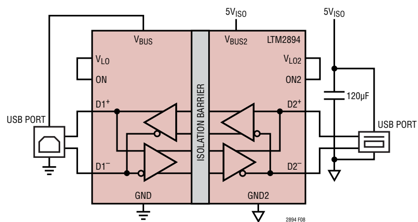
Figure 8. Bus Splitter
