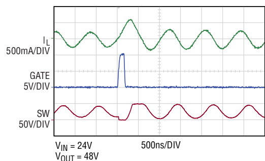
MINIMUM ON-TIME AT LIGHT LOAD WITH BLANK = SGND
