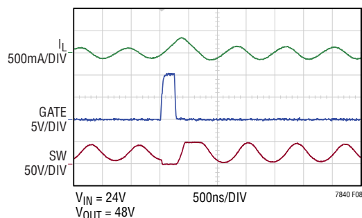
MINIMUM ON-TIME AT LIGHT LOAD WITH BLANK = INTV CC
