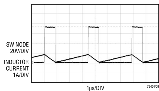
75% MAXIMUM DUTY CYCLE WITH D_{MAX} = INTV_{CC}
