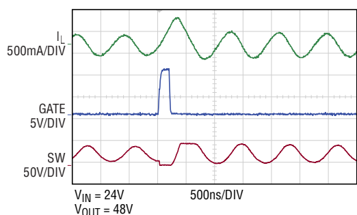
MINIMUM ON-TIME AT LIGHT LOAD WITH BLANK = FLOAT
