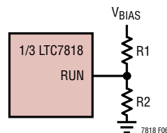
Figure 6. Using the RUN Pins as a UVLO
