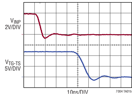
LTC7004 Driving a 1nF Capacitive Load
