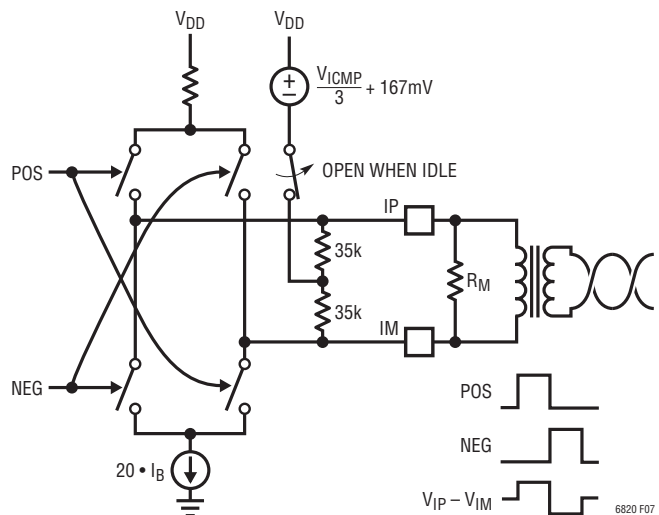
Figure 7. Pulse Driver
